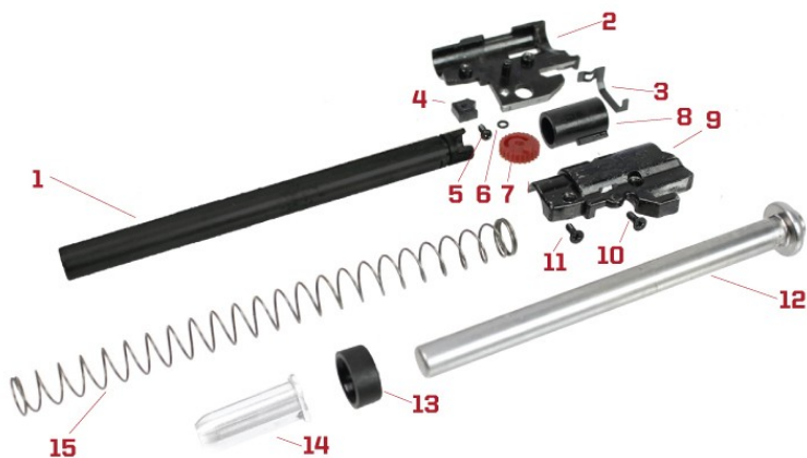
PG4-HXAB : HOP-UP UNIT & RECOIL ROD
