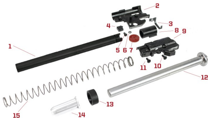
PG4-HXAB : HOP-UP UNIT & RECOIL ROD
